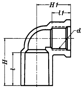
龍L接頭(塑膠牙) Faucet Fitting — 90° Elbow (Plastic Thread) 單位：mm
